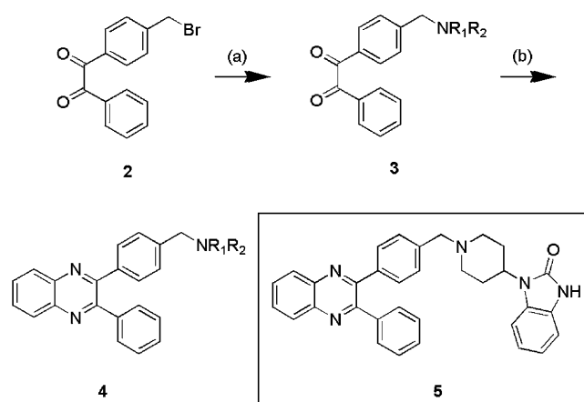
Scheme 1. Synthesis of amino-functionalized quinoxalines 4 . Reagents and conditions: (a) (i) HNR_1R_2 , PS-DIEA, DCM, rt, (ii) R_1-SH , (iii) Fluorot Flash TM SPE, 62–95%; (b) 1,2-diaminobenzene, EtOH/HOAc (9:1), 160 °C, 10 min, microwave, 89–99%. All compounds purified by mass-guided HPLC. 10
