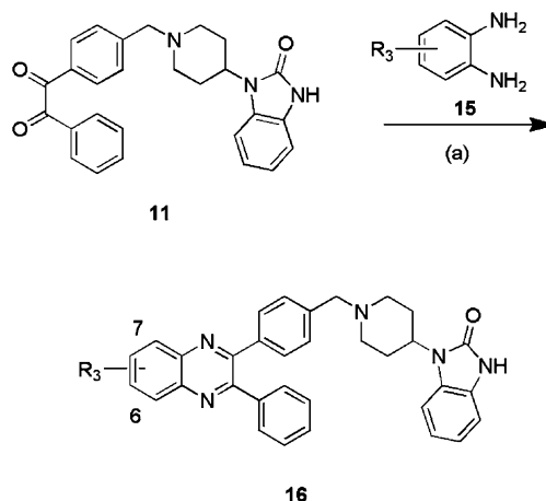
Scheme 3. Synthesis of functionalized quinoxalines 16 . Reagents and conditions: (a) EtOH/HOAc (9:1), 160 °C, 10min, microwave, 85–99%. All compounds purified by mass-guided HPLC. 10
