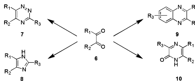
Figure 3. 1,2-Diketone approach to diverse heterocycles.
